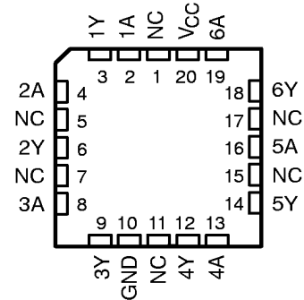
SN54LV05A . . . FK PACKAGE (TOP VIEW)
