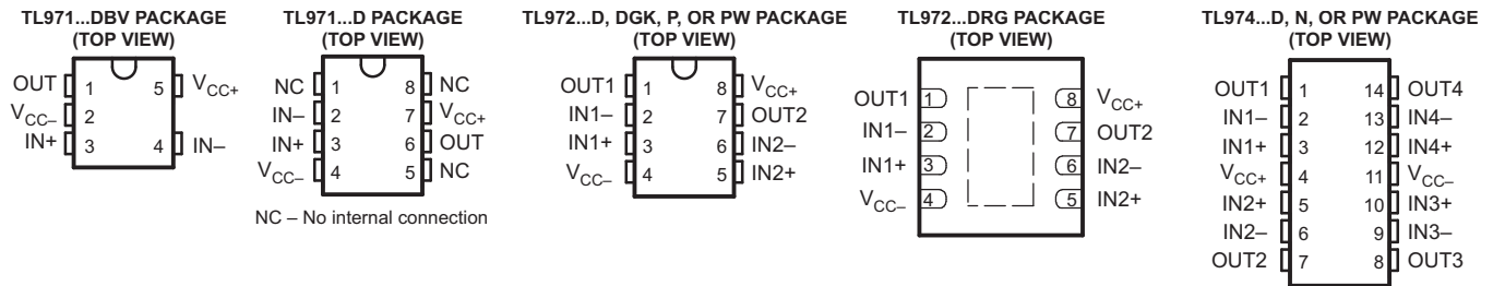
Pin Functions
