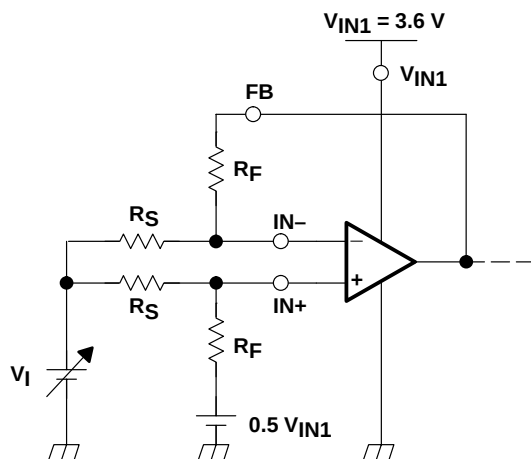
Figure 3. V_{ICR}
