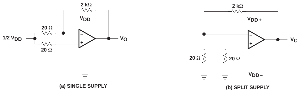
Figure 36. Noise-Test Circuit
