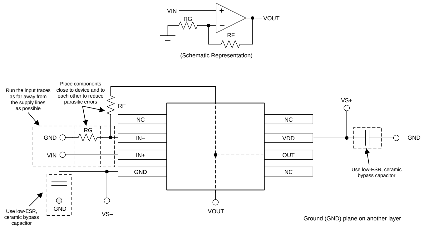
Figure 31. TLV27x Layout Example
