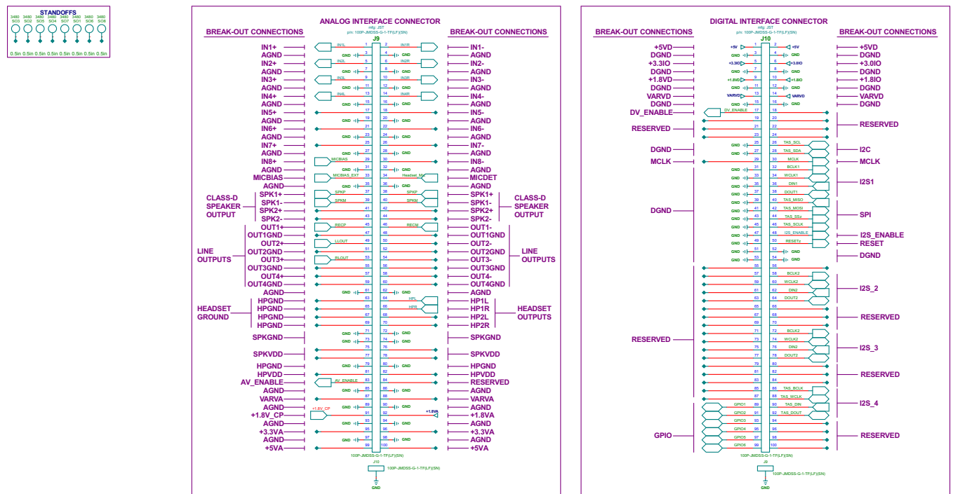
Figure B-8. Analog and Digital Interface Connectors
