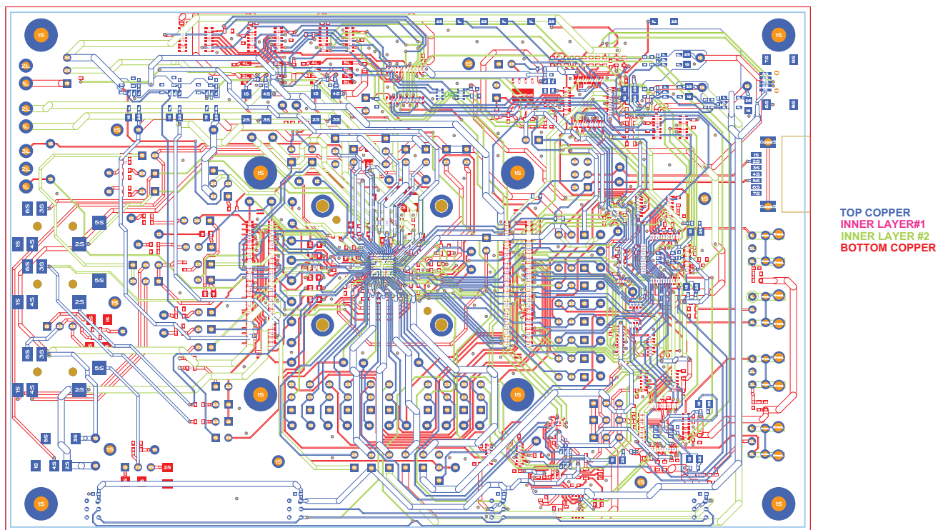
Figure C-3. Routing
