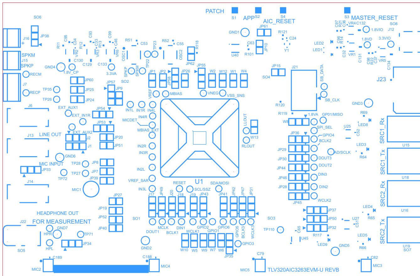
Figure C-1. Silkscreen Top
