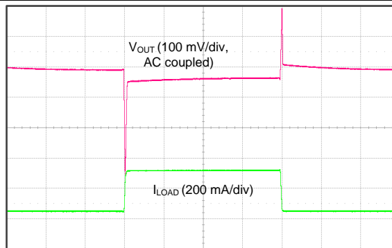
Figure 26. 1.0 V, 50-mA to 300-mA Load Transient
