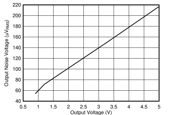
Figure 5-6. Output Noise Voltage vs V_{OUT}
