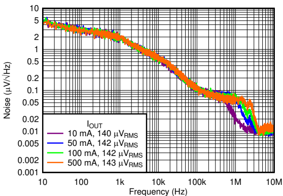
Figure 5-5. Output Spectral Noise Density vs Frequency and I_{OUT}
