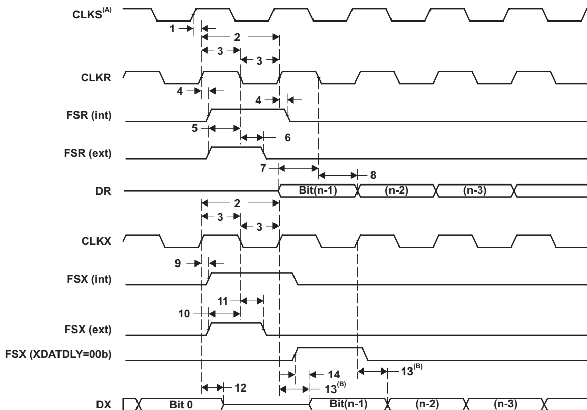
Figure 7-36 McBSP Timing
