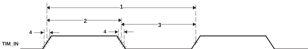
Figure 6-73. Timer Timing
