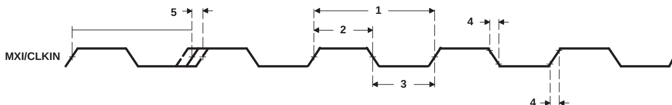
Figure 6-15. M24XI Timing
