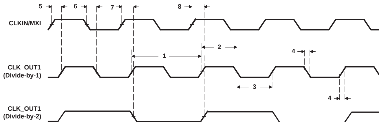
Figure 6-17. CLK_OUT1 Timing
