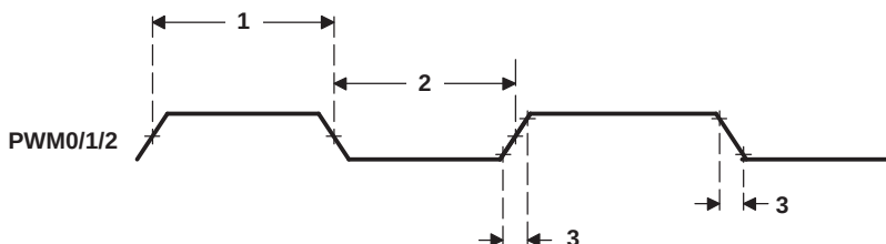
Figure 6-74. PWM Output Timing
