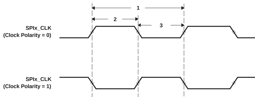
Figure 6-61. SPI_CLK Timing
