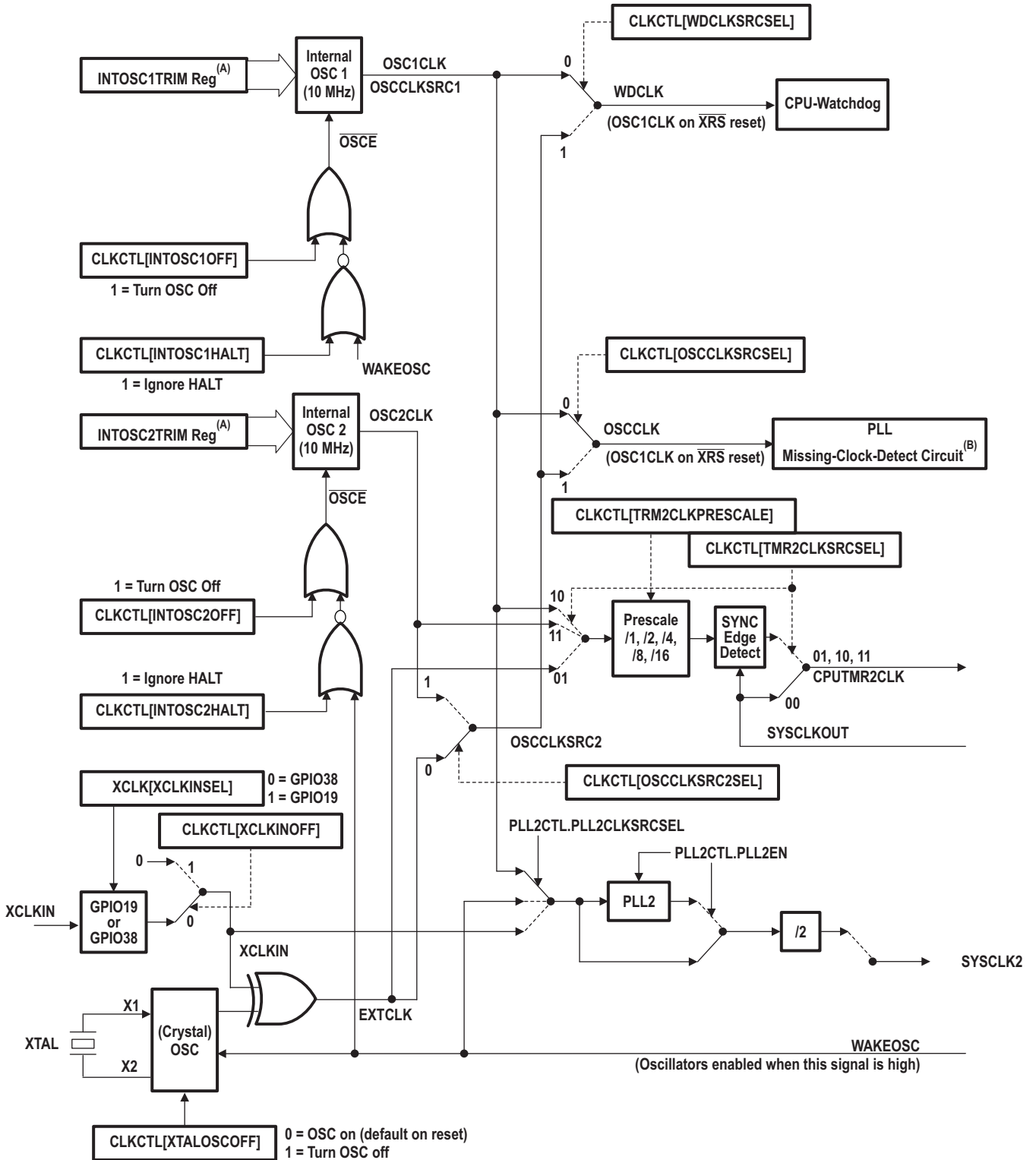
Figure 5-5. Clock Tree
