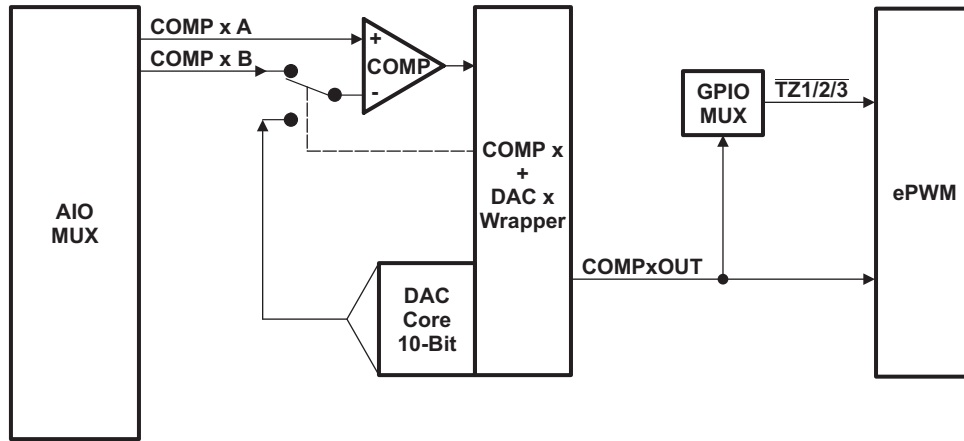
Figure 5-22. Comparator Block Diagram
