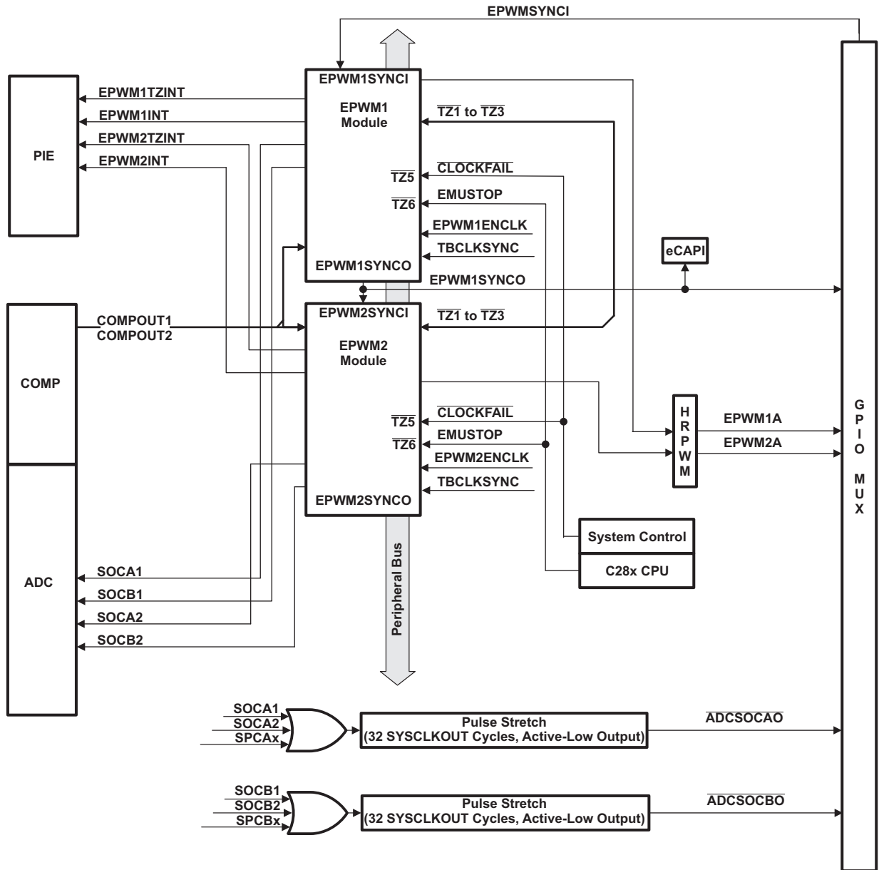
Figure 5-38. ePWM
