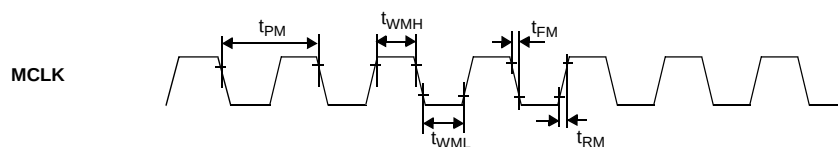
FIGURE 3. MCLK Timing
