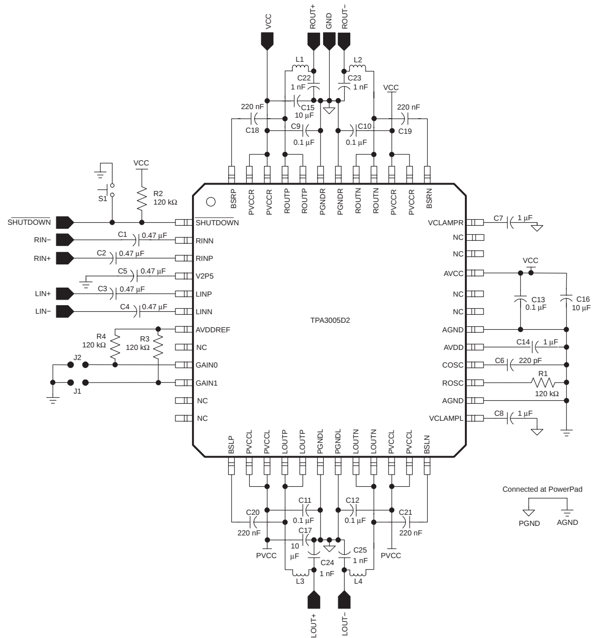
Figure 3–1. TPA3005D2EVM Schematic
