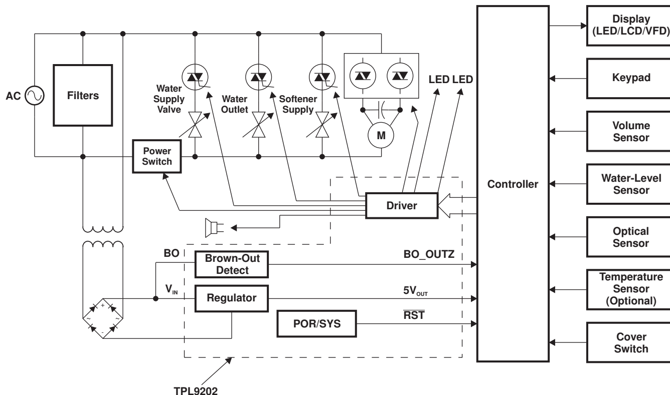
Figure 3. Washing-Machine Application
