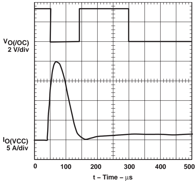
Figure 3. Short-Circuit Response, Short Applied to Powered-on 5-V xVCC-Switch Output
