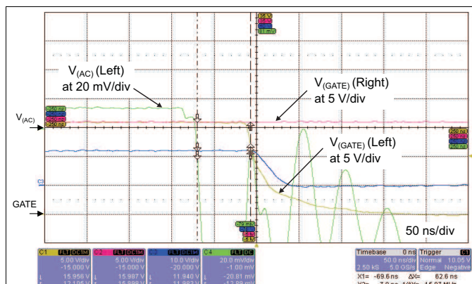
Figure 12. Typical Turnoff With Two ORED Devices Active ( V_{DD} = 12 V, I_{(LOAD)} = 5 A, IRL3713, Transient Applied to Left Side)
