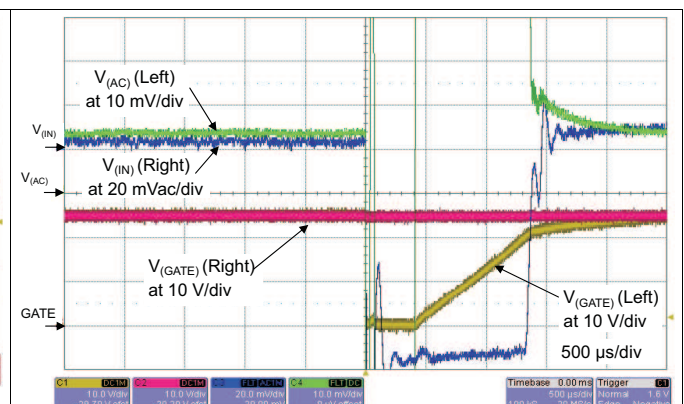
Figure 13. Typical Turnoff And Recovery With Two ORED Devices Active ( V_{DD} = 3 V, V_A = 18 V, I_{(LOAD)} = 5 A, IRL3713, Transient Applied to Left Side)
