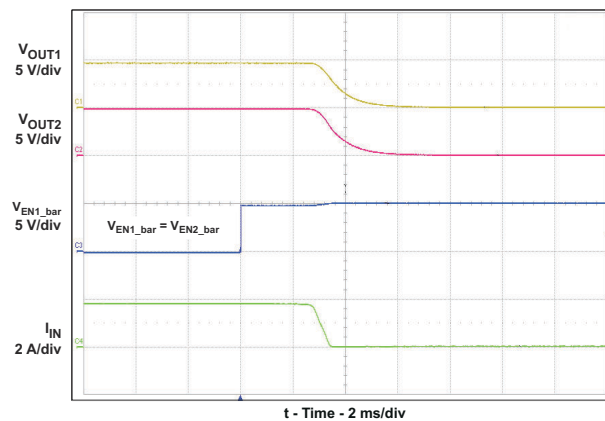
Figure 10-7. Turn-Off Delay and Fall Time
