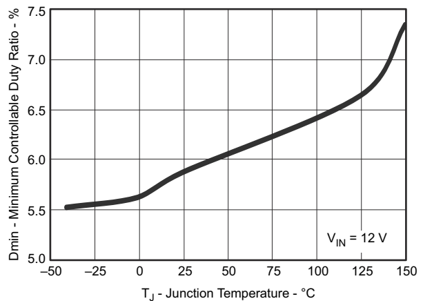
Figure 6-6. Minimum Controllable Duty Ratio vs Junction Temperature
