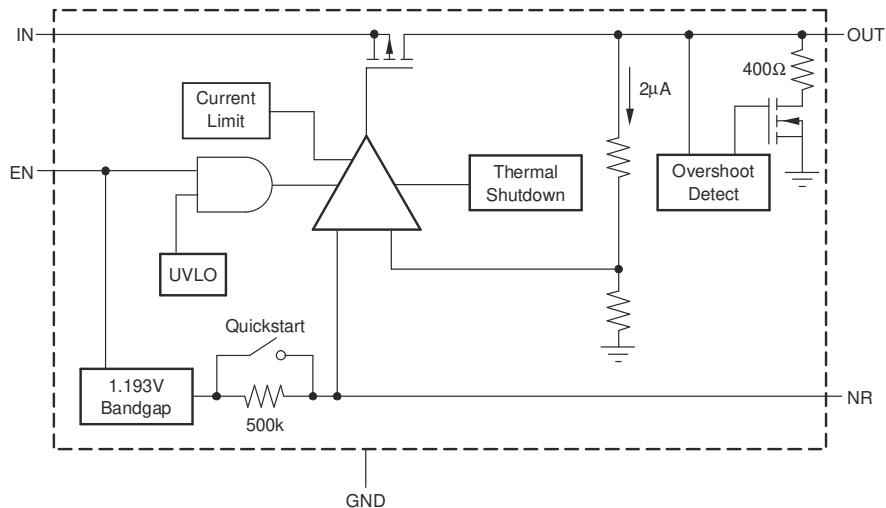
Figure 7-1. Fixed-Voltage Versions
