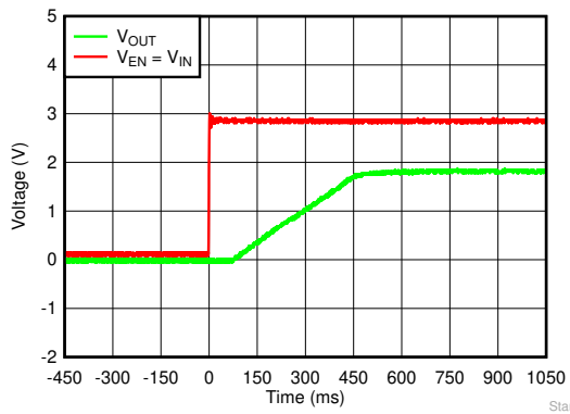
V_{OUT} = 1.8\text{ V} , I_{OUT} = 200\text{ mA} , C_{OUT} = 1\text{ }\mu\text{F}
