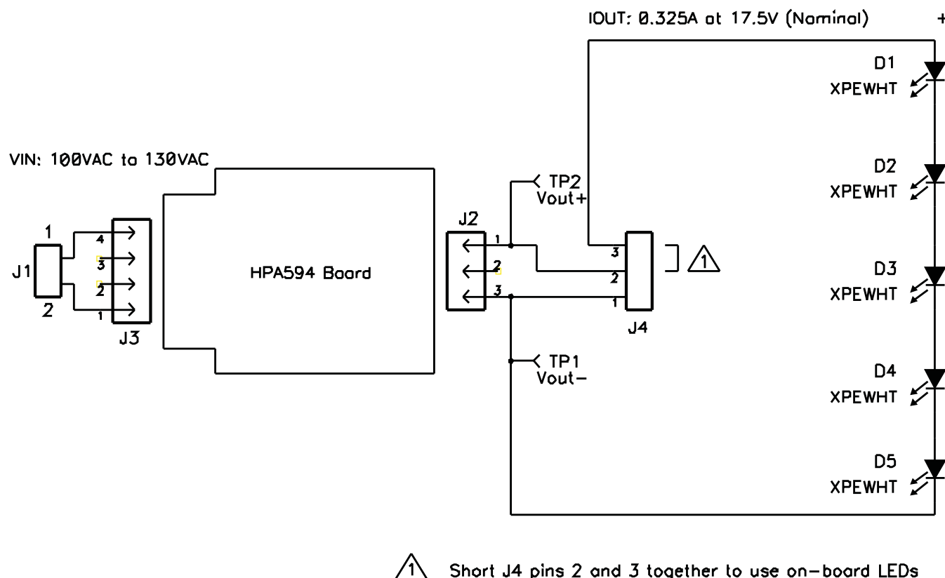
Figure 2. TPS92010EVM-592 LED Load Board Schematic
