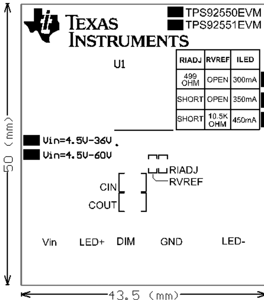
Figure 42. Top Overlay
