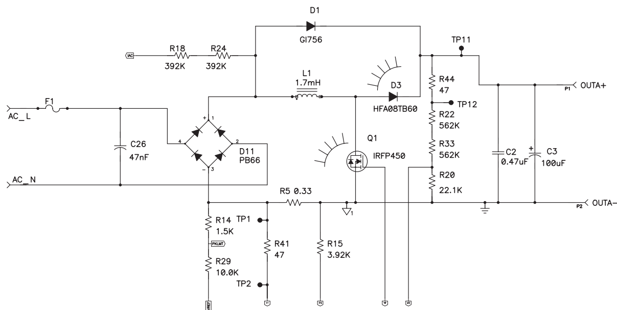
Figure 5. Section A
