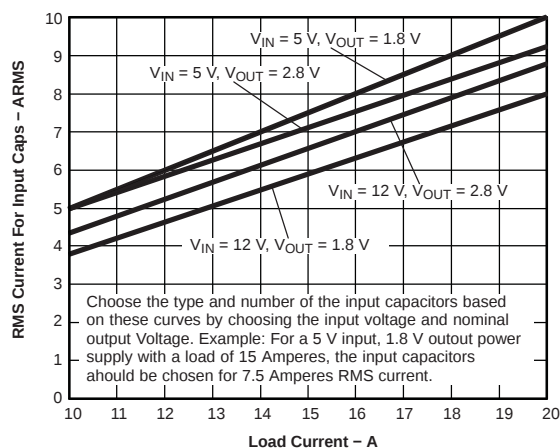
Figure 8. Load Current vs RMS Current for Input Capacitors – Pentium® II Family
