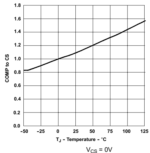
Figure 6-4. COMP to CS Offset Voltage vs Temperature V_{CS} = 0V
