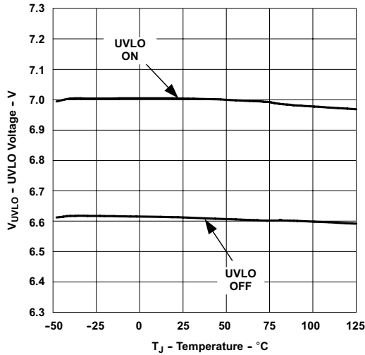
Figure 6-11. Undervoltage Lockout vs Temperature
