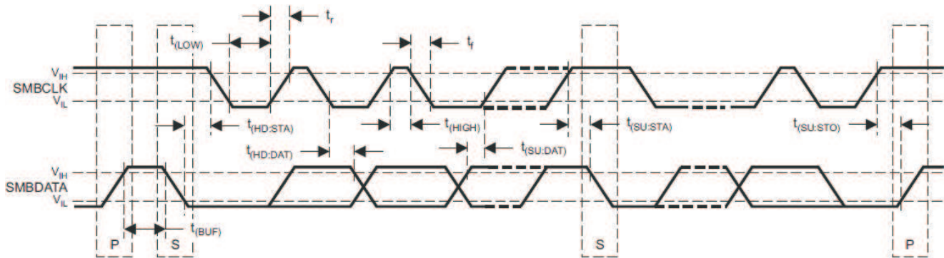
Figure 5-1. I²C/SMBus/PMBus Timing Diagram
