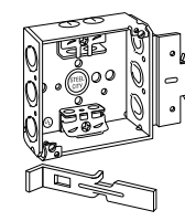
52151 MS X* MS bracket for 1/4", 2/4", 3/4", 4" metal studs
