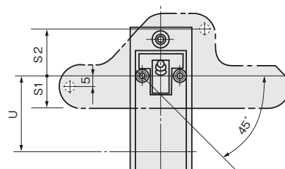
Shape of cam for THA-203-4-THA-109-3
