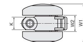
TY40N□S / TY50N□S (with stopper)
