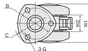
TY40S / TY50S (with stopper)
