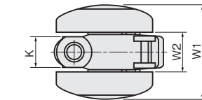
TY40N□S / TY50N□S (with stopper)
