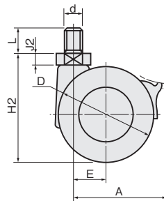
TY40S / TY50S (with stopper)
