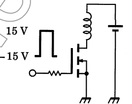
TEST CIRCUIT
