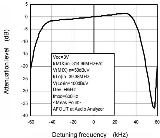
Detuning Characteristics
