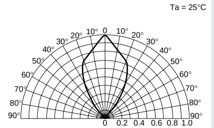
Radiation pattern
