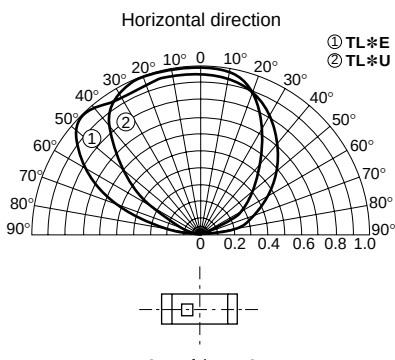
Radiation pattern
