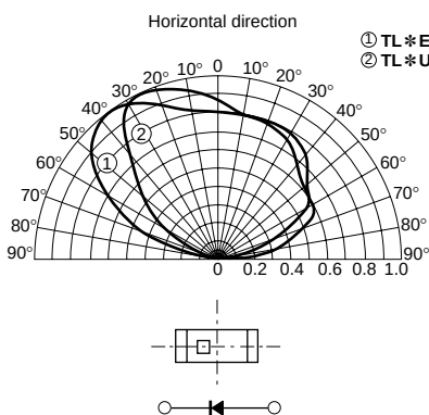
Radiation pattern
