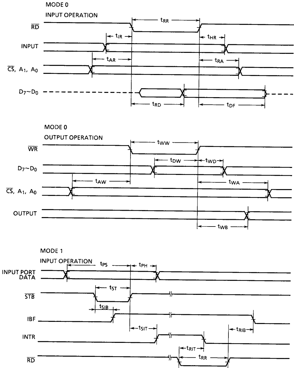
Figure 7.1 Timing diagram
