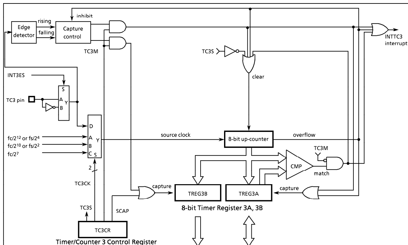
Figure 2-26. Timer/Counter 3
