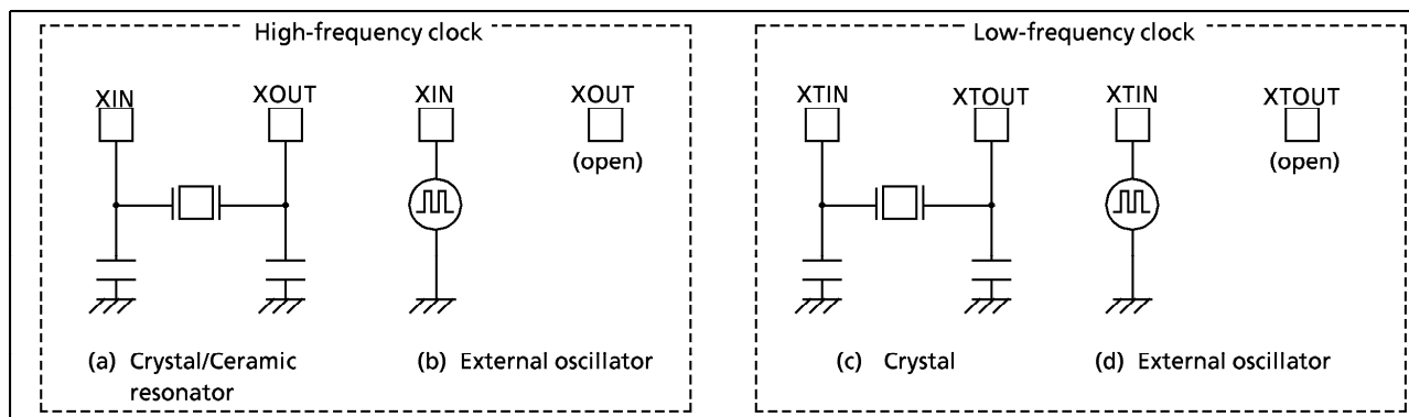
Figure 1-10. Examples of Resonator Connection
