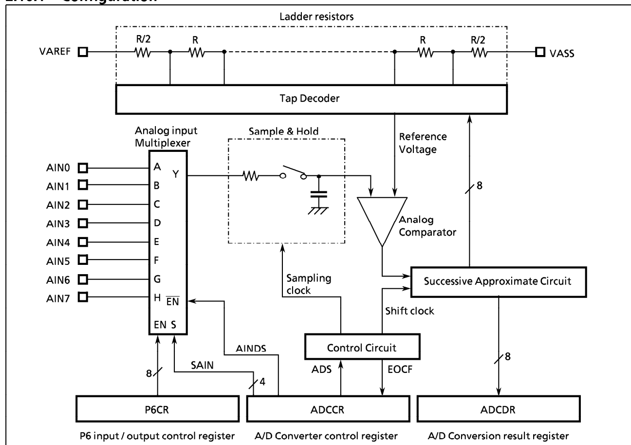
Figure 2-43. A/D Converter
