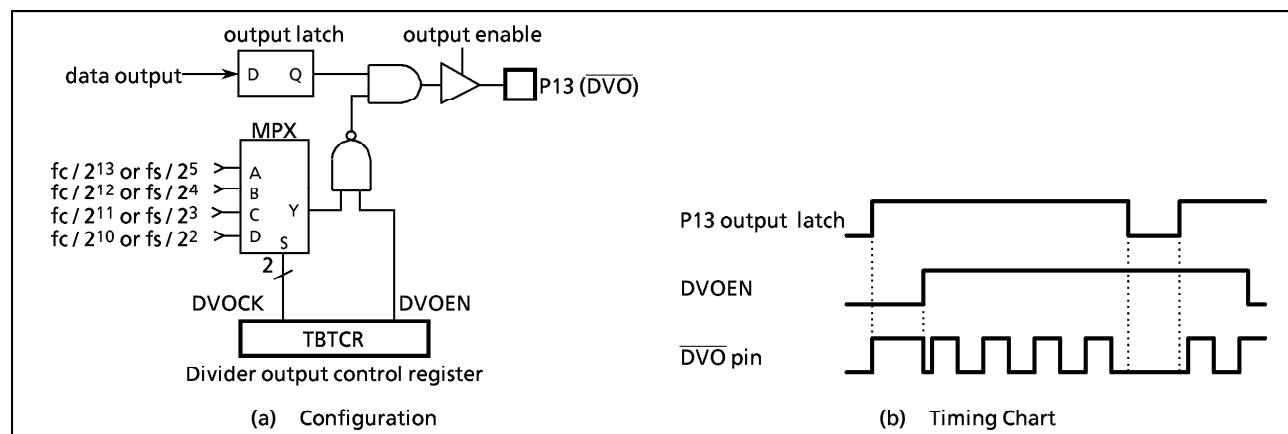
Figure 2-13. Divider Output
