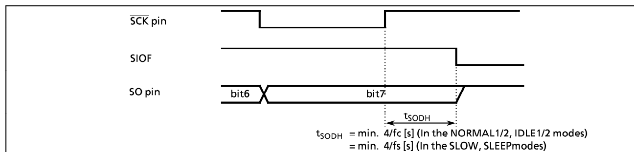
Figure 2-42. Transmitted Data Hold Time at End of Transmit/Receive
