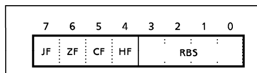
Figure 1-6. PSW (Flags, RBS) Configuration
