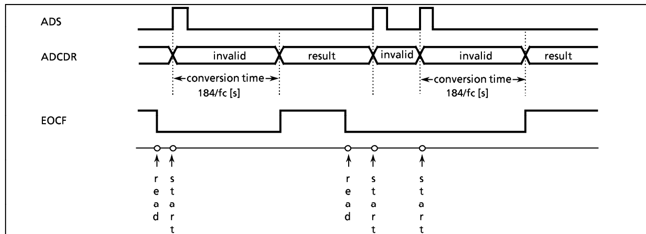
Figure 2-45. A/D Conversion Timing Chart
