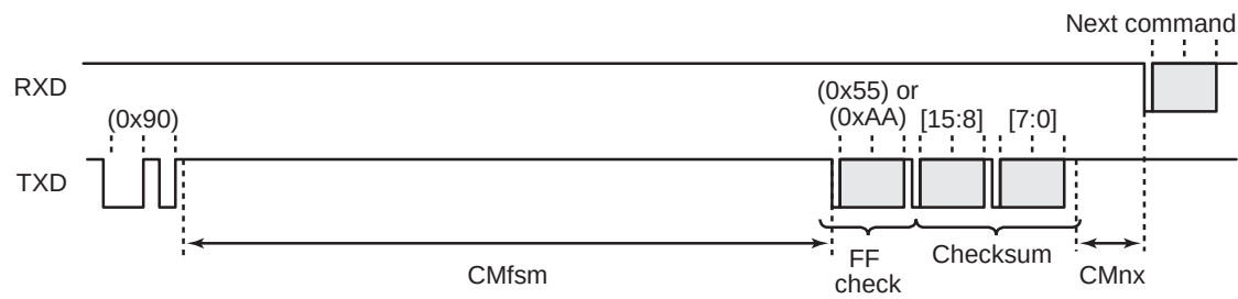
Figure 22-11 Flash Memory SUM Output Command
