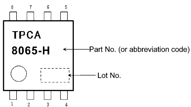
Fig. 7.1 Marking
