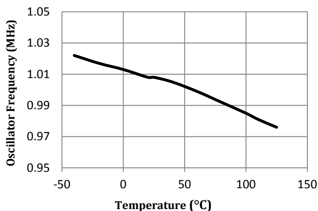
Figure 19. Oscillator Frequency vs. Temperature ( I_{out}=300\text{mA} )
