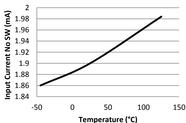
Figure 21. Input Current vs. Temperature (No load, No switching)
