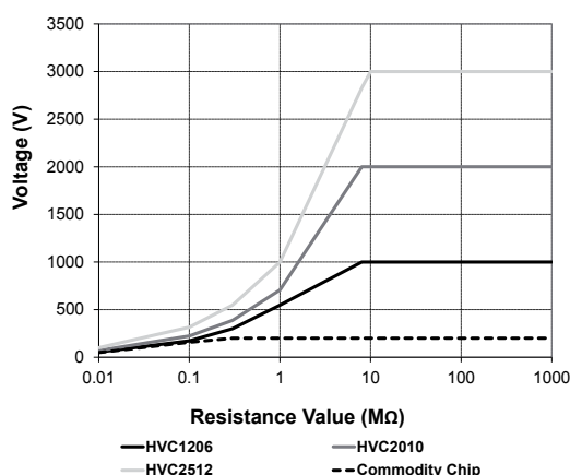
Maximum Continuous Voltage
