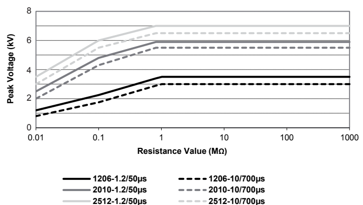
Lightning Strike Performance
