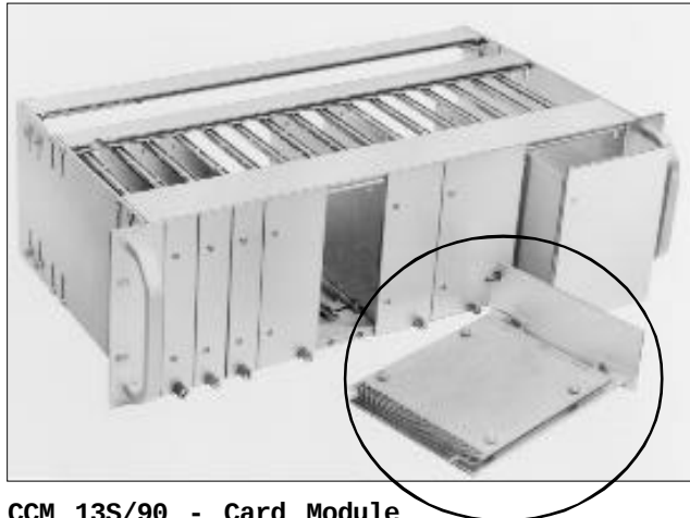
CCM 13S/90 - Card Module Rack with assorted cardmount modules
