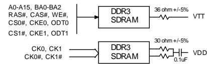
Command, address, control, and clock line terminations
