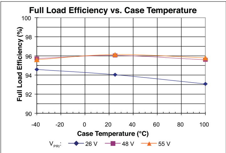
Figure 2 — Full secondary load efficiency vs. temperature
