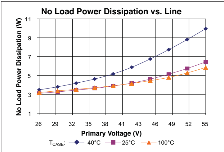
Figure 1 — No load power dissipation vs. V_{PRI}
