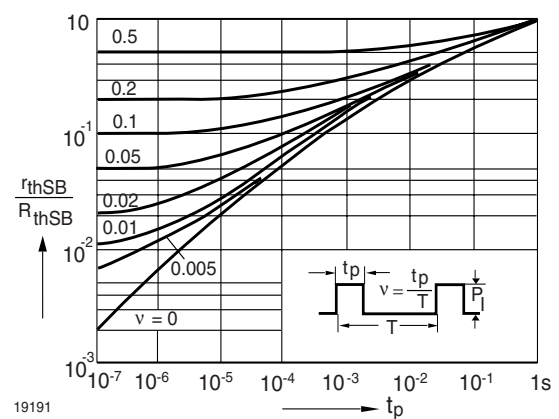
Figure 2. Pulse Thermal Resistance vs. Pulse Duration (normalized)
