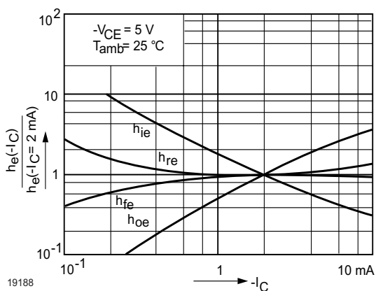
Figure 8. Relative h-Parameters vs. Collector Current
