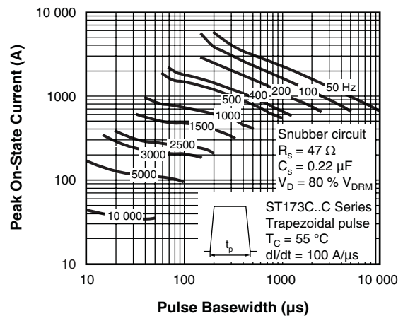
Fig. 15 - Frequency Characteristics
