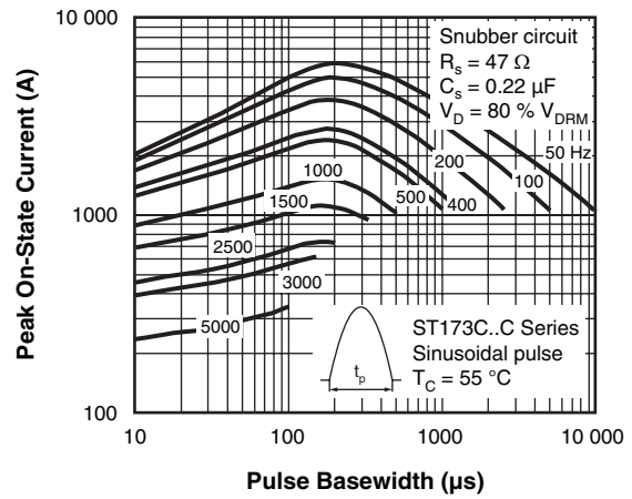
Fig. 13 - Frequency Characteristics
