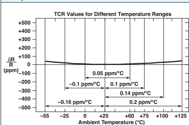
Figure 3—Typical Resistance/ Temperature Curve
