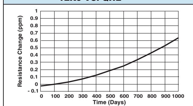
FIGURE 1 - SHELF LIFE - VHA518-11 12K9 VS. QHE
