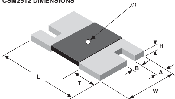
FIGURE 2 - DIMENSIONS AND IMPRINTING in inches (millimeters)
