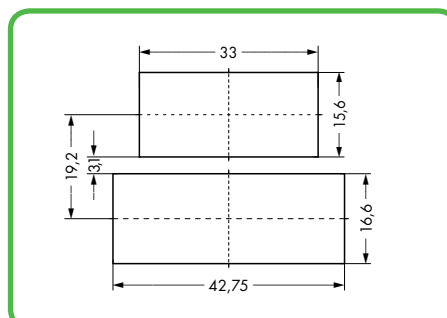
If the 7-pole strain relief housing is used with snap-in connectors, the sheet cutouts have to be made as described above.
