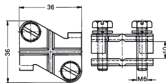
Dimensions for clamping yoke AK 95
