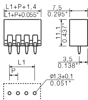
Dimensioned drawing
