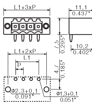
Dimensioned drawing
